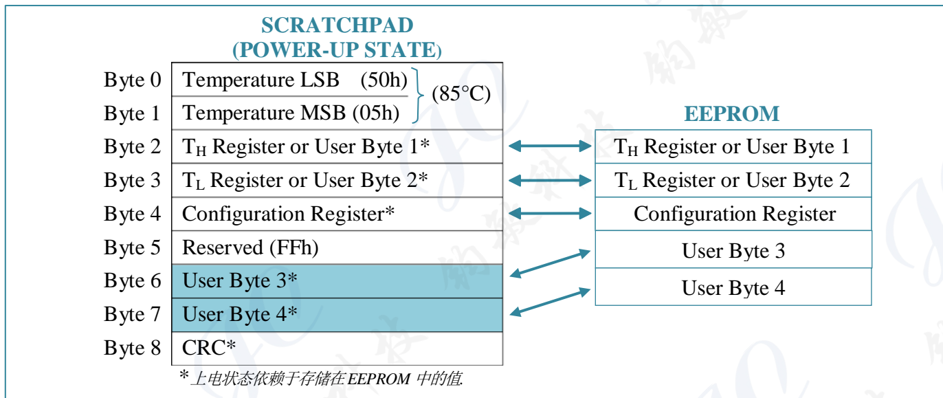
Figure 7. GX18E20 Memory Map
