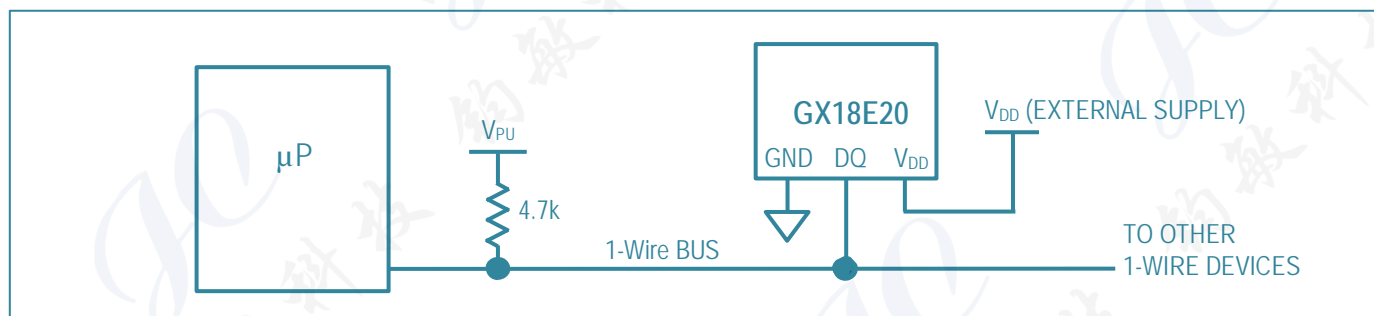
Figure 5. Powering the GX18E20 with an External Supply
