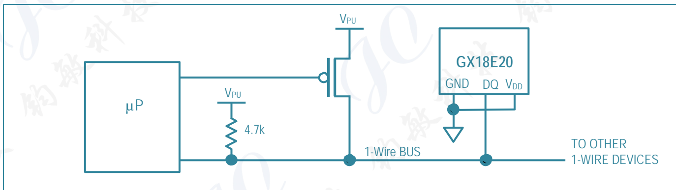
Figure 4. Supplying the Parasite-Powered GX18E20 During Temperature Conversions
